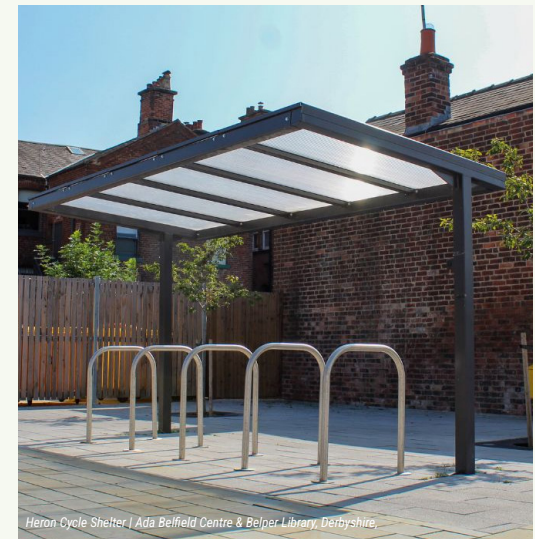
Heron Cycle Shelter | Ada Bellfield Centre & Belper Library, Derbyshire
